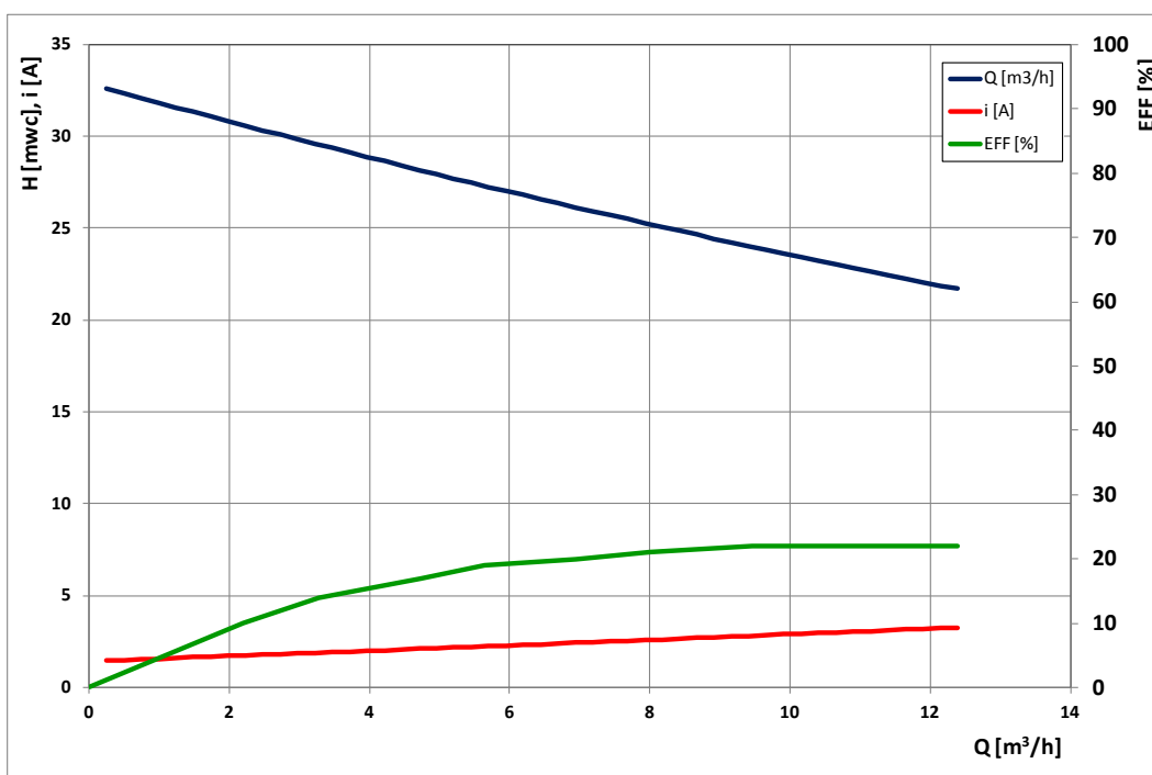
Curva – Curve
