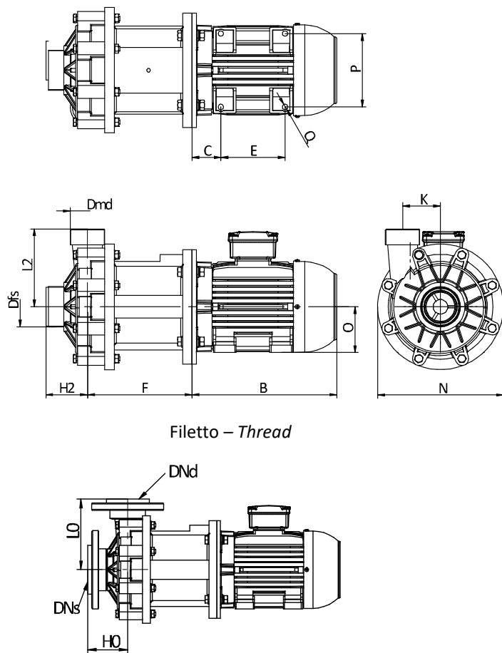
Flangia libera – Backing ring
