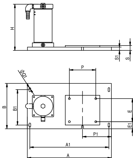
Lato pompa - Pump side
